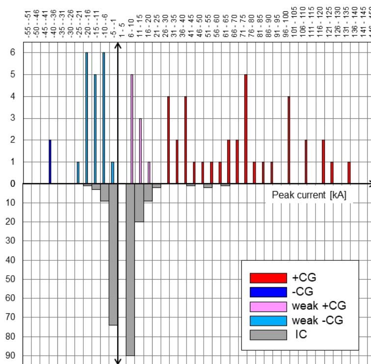
Fig. 5. Histograms of JLDN-detected sferic events versus peak current in the eyewall of the decaying stage of T1915. Sferics identified as CG events are shown in the upward histograms, with positive events on the right and negative events on the left. Much more numerous IC events are shown in the downward filled gray bars (note vertical scale difference).
