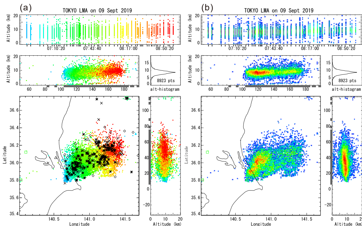
Fig. 4. Overview of the lightning activity in the eyewall of the decaying stage of T1915, as determined by the Tokyo LMA. Fifty-five lightning flashes occurred over a 2-h and 15-min time period. a) Temporal progression of the VHF sources. b) Logarithmic density of the sources. Triangle, cross, diamond, and star marks in the plan views indicate the location of -CG , +CG , -IC , and +IC events detected by JLDN, respectively (shown as gray bars at the base of the vertical projection panels). Square green symbols at the left edge of the plan panels indicate two easternmost Tokyo LMA stations. (Plots utilize solutions from six or more stations).
