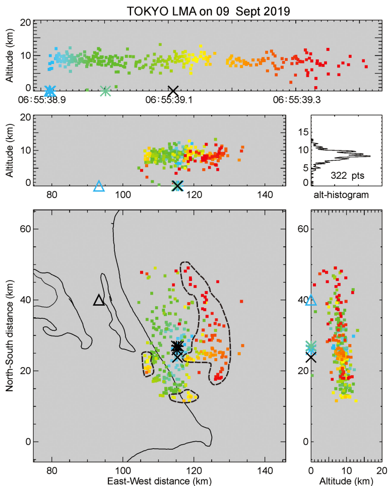
Fig. 6. VHF lightning sources for a +CG flash at 06:55:38 JST on September 9 that produced a 117-kA +CG discharge 200 ms into the flash (black X symbol). Arrival of ground potential within the cloud initiated characteristic “blooming” of the breakdown in different directions away from the extremities of the preceding activity, including an entirely new branch to the east and north (dashed areas). Triangle, cross, and star marks indicate the location and time of -CG, +CG, and +IC events detected by JLDN, respectively. (Plot shows sources located by six or more stations with chi-square values \leq 5 ).
